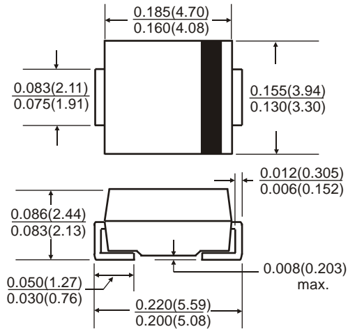
All dimensions inches and (millimeters)
